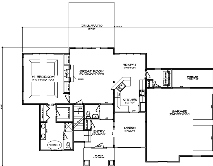
FIRST FLOOR PLAN A-4
