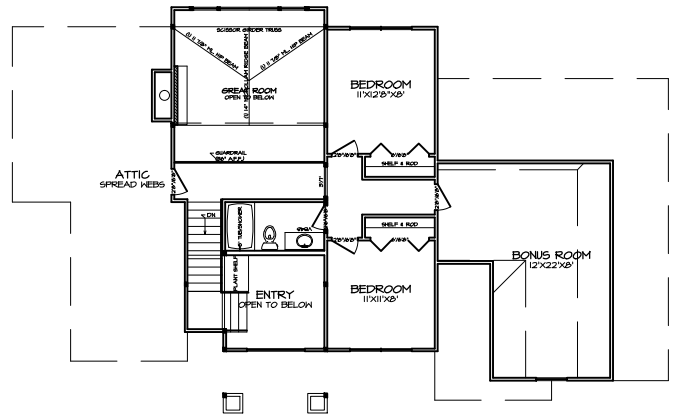
SECOND FLOOR PLAN A-5
